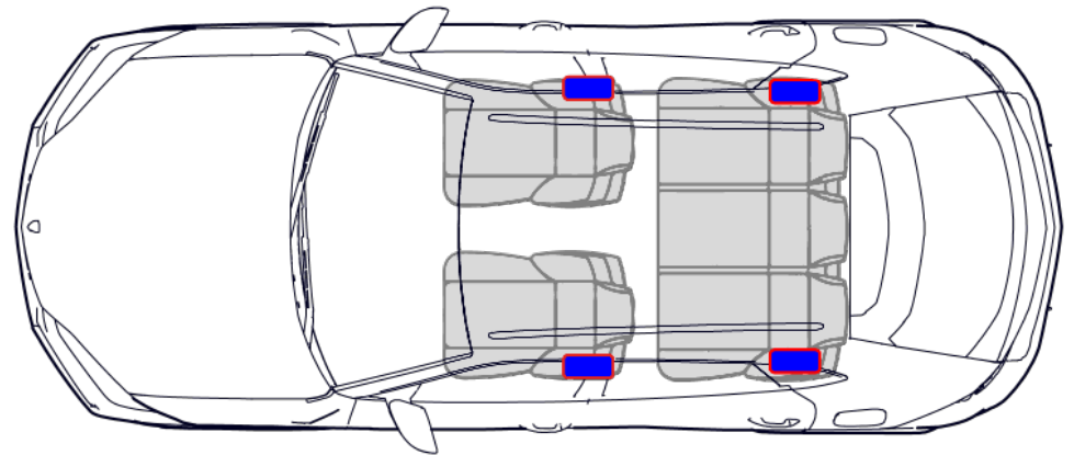
Side airbags position
